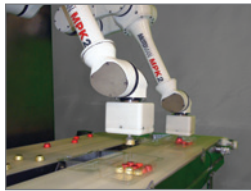
Conveyor Tracking
