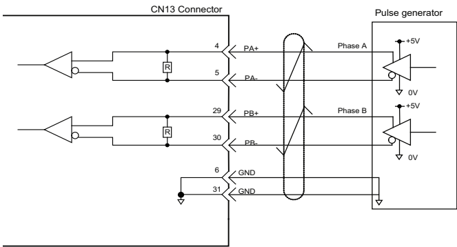
Encoder Input Circuit
