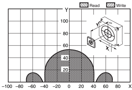
V680-HS63 (mounted on metallic material) & V680-D8KF68/-D32KF68 (mounted on non-metallic material) (Tag direction: Horizontal) V680-HS63 (mounted on metallic material) & V680-D8KF68/-D32KF68 (mounted on non-metallic material) (Tag direction: Vertical)
