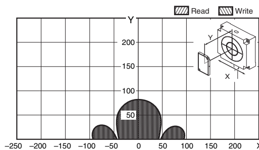
V680-H01-V2 (mounted on non-metallic material) & V680-D8KF68/-32KF68 (Tag direction: Vertical)
