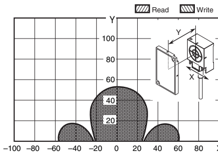
V680-HS65 (mounted on metallic material) & V680-D8KF68/-D32KF68 (mounted on non-metallic material) (Tag direction: Vertical)
