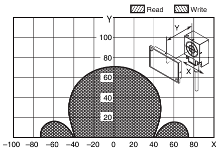
V680-HS63 (mounted on metallic material) & V680-D8KF68/-D32KF68 (mounted on metallic surface: steel) (Tag direction: Horizontal) When the V680-A81 attachment is mounted on RF Tag
