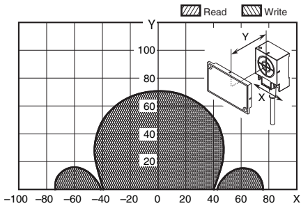
V680-HS63 (mounted on metallic material) & V680-D8KF68/-D32KF68 (mounted on metallic surface: steel) (Tag direction: Horizontal) V680-HS63 (mounted on metallic material) & V680-D8KF68/-D32KF68 (mounted on metallic surface: steel) (Tag direction: Vertical)
