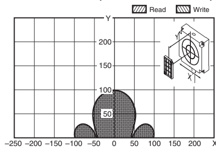
V680-HS65 (with Metal on Back Surface) & V680S-D2KF68M (Metal on back: Steel) (Tag direction: Horizontal) V680S-D2KF68M (Metal on back: Steel) (Tag direction: Vertical)
