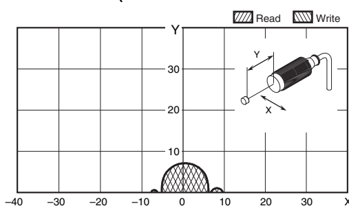
V680-HS51 (embedded in metallic material) & V680-D2KF52M (embedded in metallic surface: steel)
