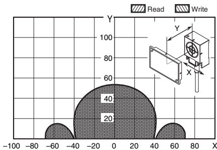
V680-HS65 (mounted on metallic material) & V680-D8KF68/-D32KF68 (mounted on non-metallic material) (Tag direction: Horizontal)
