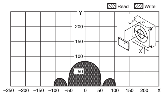
V680-H01-V2 (mounted on non-metallic material) & V680-D8KF68/-D32KF68 (Tag direction: Horizontal)
