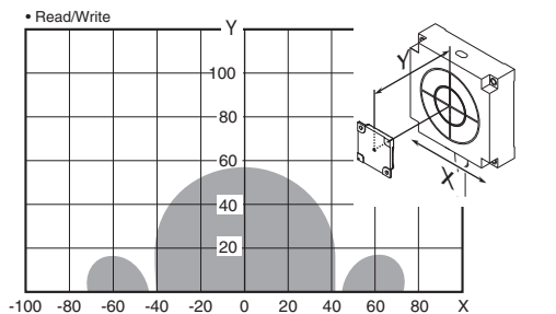
V680-HS63 (mounted on non-metallic material) & V680S-D8KF68 (Tag direction: Horizontal)
