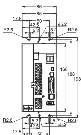
External dimensions
