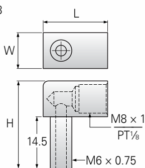
OB-M6-M8 (PT \frac{1}{8} )
