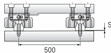
Permissible Tolerance (S) for Two Level
