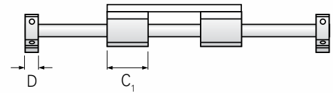
Double Shaft End Supported with 4 Pillow Blocks and Carriage 1
