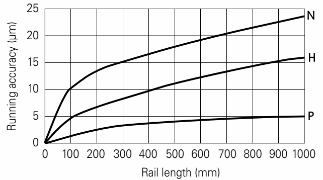
Accuracy of the running parallelism
