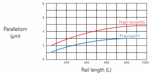
Rail length and parallelism of rolling plane
