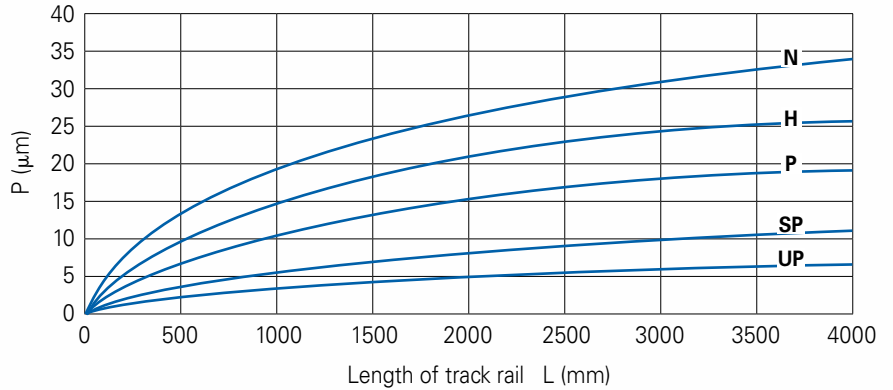
ACCURACY OF RUNNING PARALLELISM
