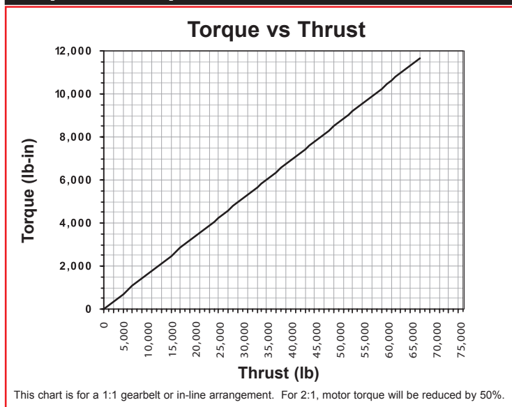
Graph 2: Torque Vs. Thrust at Ball Screw
